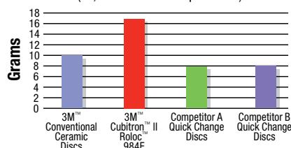
Total Cut Cubitron II Roloc 984F vs. Conventional Ceramic (3", Grade 80/80+ equivalents)
